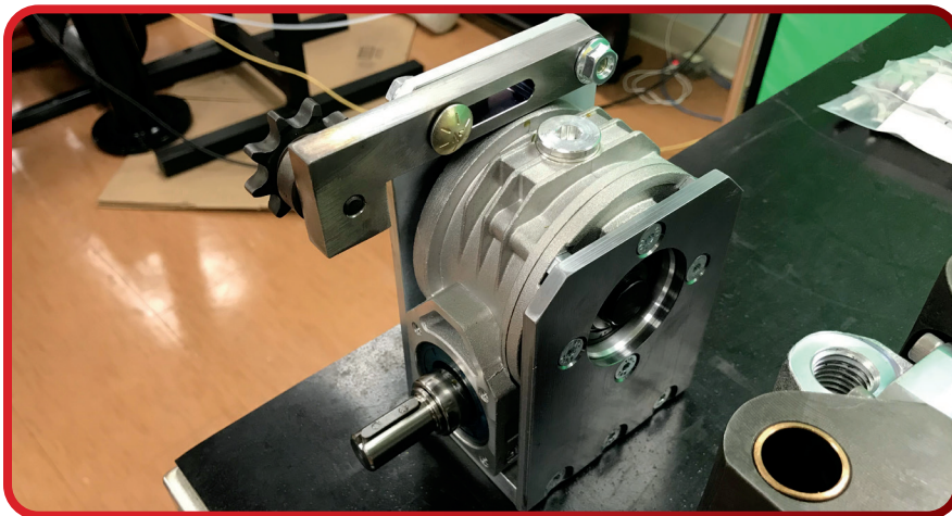
Feed Drive Assembly with Chain Tensioner
