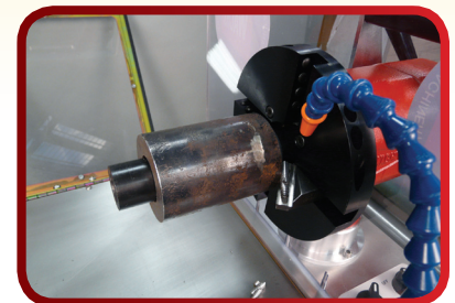
Solid build quality ensures a long service life. The heart of the Coupon Station is Wachs super rugged SDB 206/2 I.D. mount machine tool.
