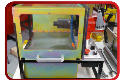
The clear enclosure helps prevent coolant splash and keeps hands away from revolving parts. An open end allows for longer pipe and coupon lengths.
